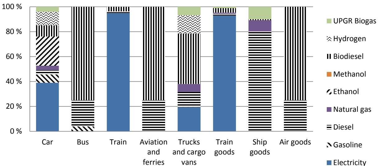
Figure 3: Fuel use in transport sector in the Carbon Neutral Scenario (CNS) 2050. Measured as fuel consumption in percent person transportation work (pkm) or percent freight transportation work (tkm)
