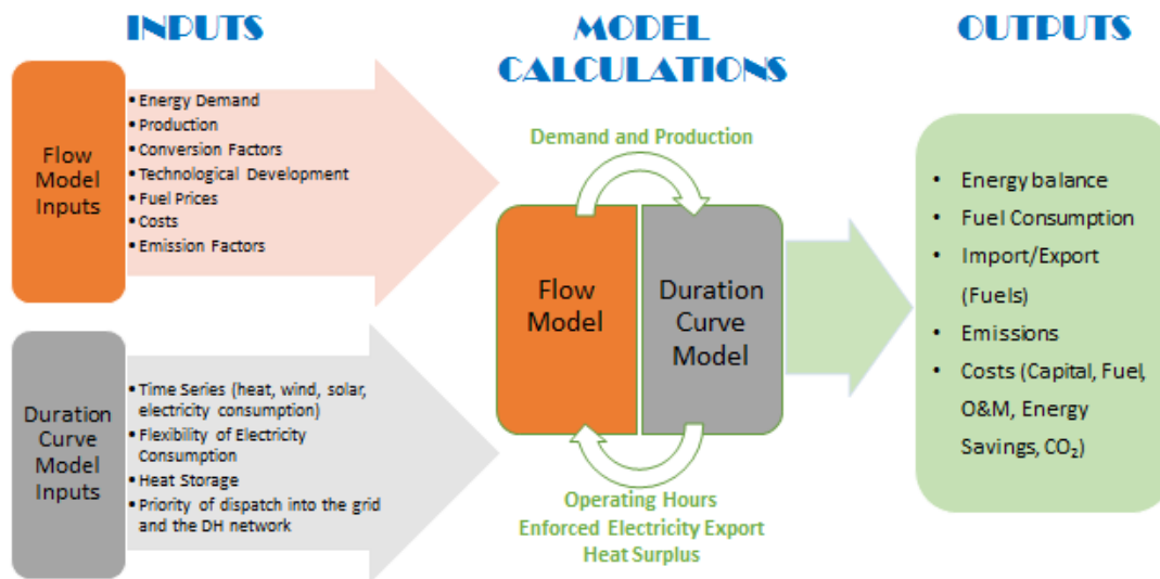
Figure 2: Linkage between Flow Model and Duration Curve Model in STREAM [12]
