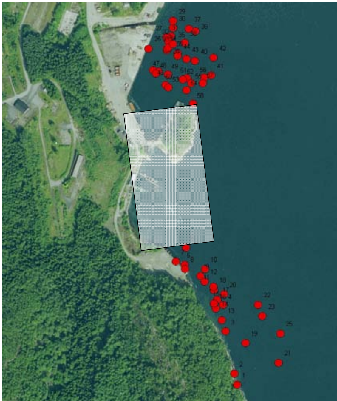
Figure 3.. Registered anthropogenic material at AF Miljøbase Vats. See Table 9 for description of each numbered point. Please observe that the aerial photograph was taken before the recent constructions were finalized. The grey area gives a coarse indication of the area now filled in.
